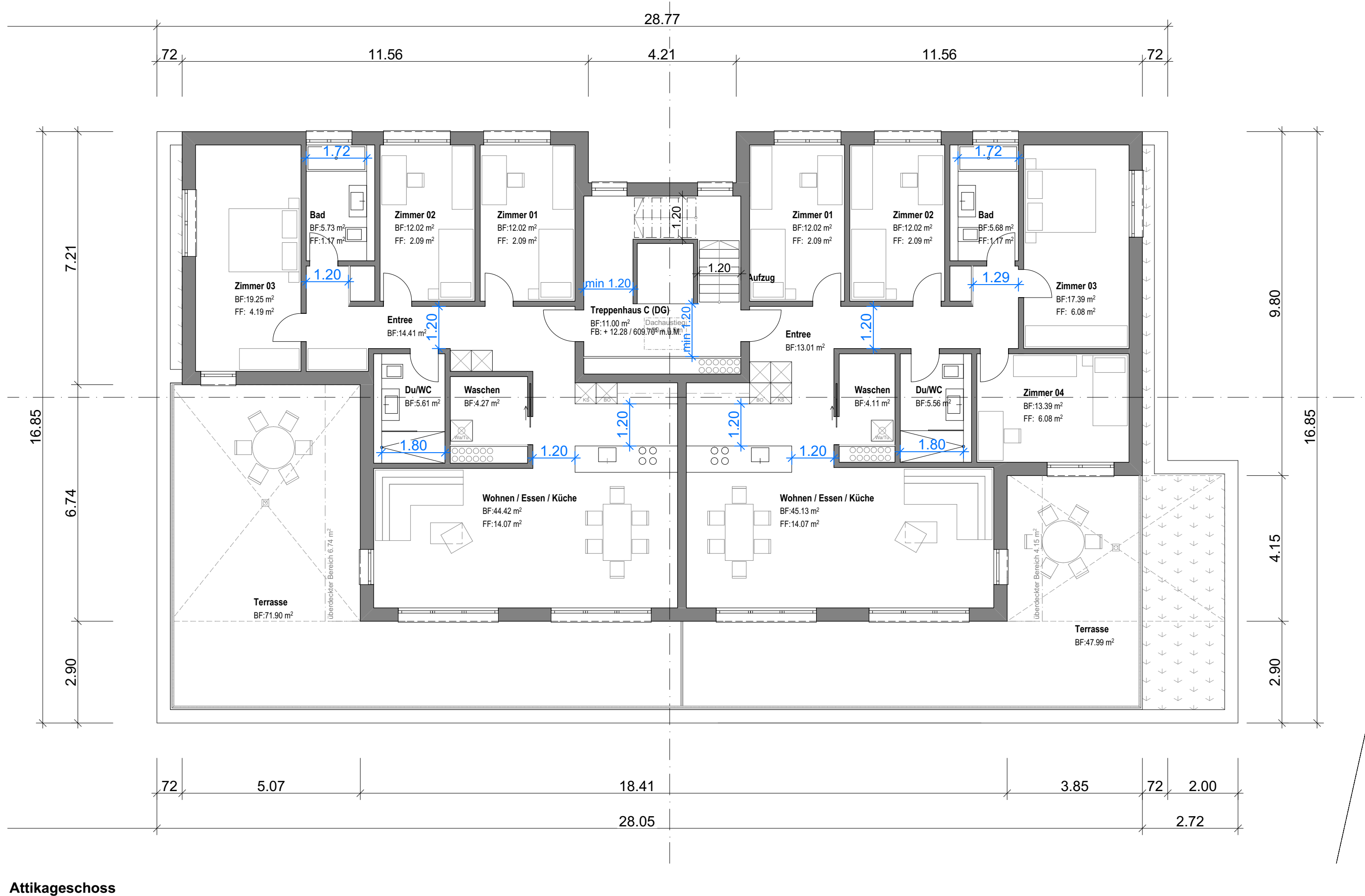
Attikageschoss
